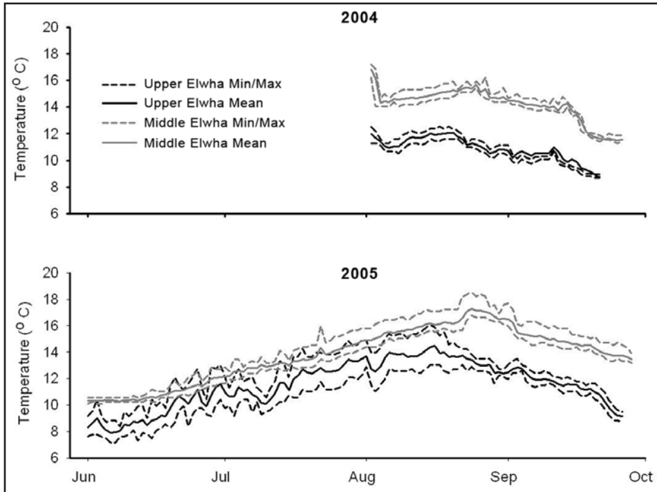
Figure 4. Minimum, mean, and maximum water temperatures ( ^{\circ}\text{C} ) in the middle and upper Elwha River, 2004 and 2005.
