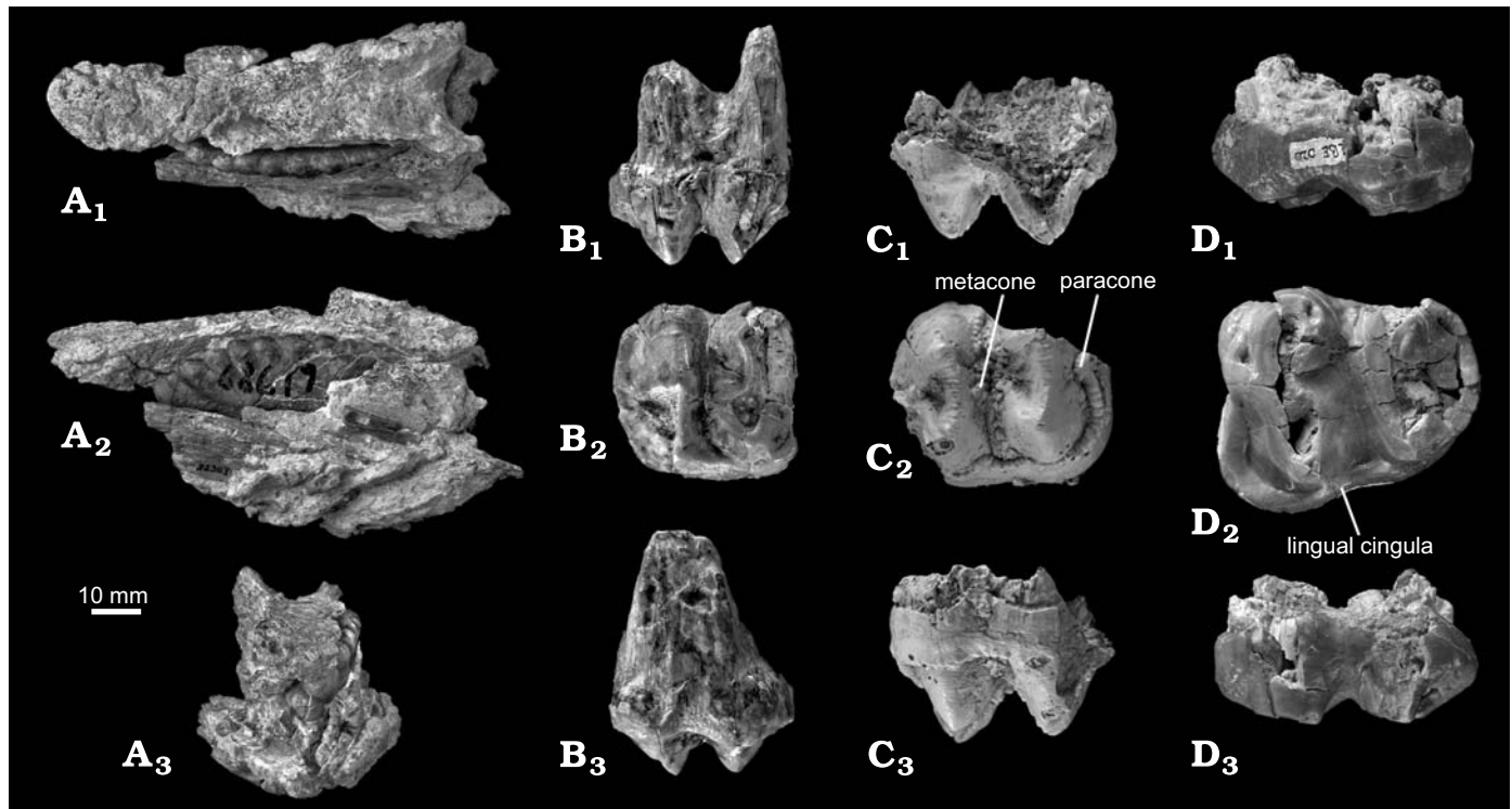
Fig. 3. Dental elements of the proboscidean Arcanothorium savagei (Court, 1995), from the Evaporite (A and C, late Eocene) and Idam (B, early Oligocene) units of Dor El Talha, Libya. A. Erupting left i1 (BMNH M. 82183) in occlusal (A 1 ), lateral (A 2 ), and anterior (A 3 ) views. B. Right M1 (BMNH M. 82172) in buccal (B 1 ), occlusal (B 2 ), and lingual (B 3 ) views. C. Right M2 (BMNH M. 82398) in buccal (C 1 ), occlusal (C 2 ), and lingual (C 3 ) views. D. Left M3 (MNHN LBE 20) in buccal (D 1 ), occlusal (D 2 ), and lingual (D 3 ) views.
