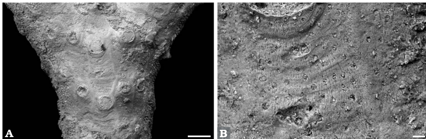
Fig. 10. Multisparisid cyclostome bryozoan Idmonea sp. from the Middle Jurassic ore-bearing clays of the Polish Jura, GIUS 8-3509-19. A. Autozooids. B. Pseudopores. Middle Bathonian ( Morrisiceras morrissi Zone), Gnaszyn Dolny. Scale bars: 200 µm (A), 20 µm (B). BSE SEM images of uncoated specimens.
