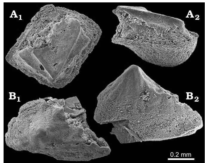
Fig. 5. Indeterminable acanthodians, SEM micrographs of micro-remains from sample S30, late Ludlow of the Niur Formation, east central Iran. A. Scale AEU 4128 in crown (A 1 ) and lateral (A 2 ) views. B. ?dentigerous jaw bone fragment AEU 4129 in occlusal (B 1 ) and lateral (B 2 ) views.
