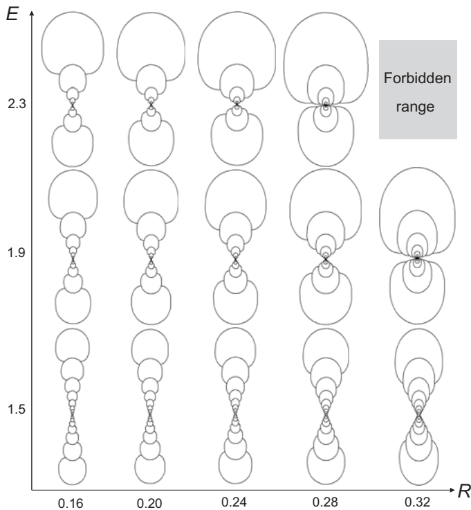
Fig. 5. Spectrum of the computer-produced ammonoids with various values of E and R when each of them is fixed throughout growth.
