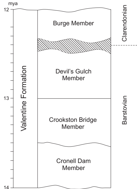
Fig. 1. Generalized stratigraphic section of the middle Miocene Valentine Formation in northern Nebraska (modified after Skinner and Johnson 1984: fig. 4 and Tedford et al. 2004: fig. 6.2). Striped area represents time gap of unconformity between members.
