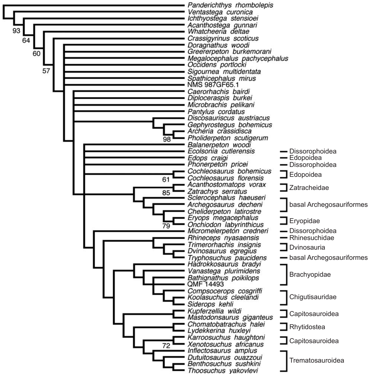
Fig. 6. Strict consensus of 38 most parsimonious trees with bootstrap percentages based upon 10,000 replicates.
