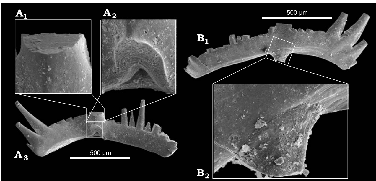
Fig. 6. SEM photographs of Sb elements of spathognathodontid conodont Lanea carlsi (Boersma, 1973). A. NM L40542, detail of cusp in cross section (A 1 ), detail of basal cavity (A 2 ), inner lateral view (A 3 ). B. NM L40543, outer lateral view (B 1 ), detail of basal area (B 2 ). All figured specimens are from sample 4Po22.
