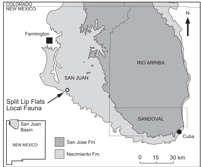
Fig. 1. Geologic map showing the the Paleocene Nacimiento Formation (Animas Formation in southern Colorado) and early Eocene San Jose Formation, San Juan Basin, New Mexico, and indicating the location of the Split Lip Flats Local Fauna.
