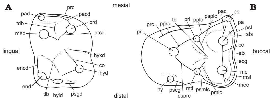
Fig. 2. Outlines of right lower molar (A) and left upper molar (B) of Chacomylus sladei gen. et sp. nov. showing tooth nomenclature used in the text. Abbreviations.—cc, centrocrista; co, cristid obliqua; ecg, ectocingulum; encd, entocristid; end, entoconid; etx, ectoflexus; hy, hypocone; hyd, hypoconid; hyld, hypoconulid; hyxd, hypoflexid; me, metacone; mec, postmetacrista; med, metaconid; msl, metastylar lobe; mtl, metaconule; pa, paracone; pac, preparacrista; pacd, paracristid; pad, paraconid; pmlc, premetaconule crista; prc, precingulum; prl, paraconule; pprc, preprotocrista; ps, parastyle; pscg, postcingulum; psl, parastylar lobe; pspic, postparaconule crista; psprc, postprotocrista; pplc, preparaconule crista; pr, protocone; prcd, protocristid; prd, protoconid; ps, parastyle; pscg, postcingulid; psl, parastylar lobe; psmlc, postmetaconular crista; st, stylocone; sts, stylar shelf; tb, talon basin; tdb, trigonid basin; tlb, talonid basin.
