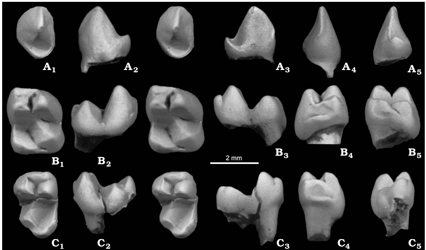
Fig. 4. Lower dentition of hypsodontid "condylarth" Chacomylus sladei gen. et sp. nov., Nacimiento Formation, lower Paleocene (late Puercan, Pu3), San Juan Basin, New Mexico. A. NMMNH P-34838, left p3? in occlusal (A 1 , stereopair), buccal (A 2 ), lingual (A 3 ), mesial (A 4 ), and distal (A 5 ) views. B. 44345, right m2 in occlusal (B 1 , stereopair), buccal (B 2 ), lingual (B 3 ), mesial (B 4 ), and distal (B 5 ) views. C. 55397, left m3 in occlusal (C 1 , stereopair), buccal (C 2 ), lingual (C 3 ), mesial (C 4 ), and distal (C 5 ) views.
