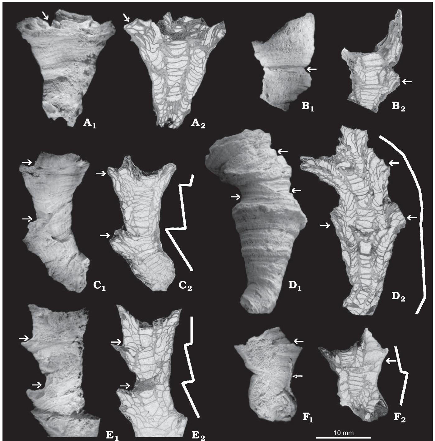
Fig. 4. External view (A 1 –F 1 ) and equivalent longitudinal sections (A 2 –F 2 ) of the studied specimens of rugose coral Catactotoechus instabilis Berkowski, 2008, Hamar Laghdad (Morocco), Emsian (Devonian). Arrows show constriction and rejuvenescence phases of growth, note on external walls they are higher than in inner part on longitudinal sections following morphology of the calice. White lines (C–F) show deflections in growth direction. A. Specimen UAM Tc/B HD3/243 showing widely expanding corallite and strong rejuvenescence in the calicular part of the corallite, note lack of dissepiments in expanding phase on the left side. B. Specimen UAM Tc/B HD 3/240 showing temporal weak constriction followed by extension phase, note markedly reduced diameter of the central lumen (aulos) caused by development of dissepiments in constriction phase. C. Specimen UAM Tc/B HD3/244 showing two weak rejuvenescences accompanying unidirectional deflections of growth. D. Specimen UAM Tc/B HD3/246 showing expansion phase followed by three weak constriction phases; note relatively gradual unidirectional deflection of growth. E. Specimen UAM Tc/B HD3/206 showing two strong rejuvenescences causing rapid unidirectional deflections of growth. F. Specimen UAM Tc/B HD3/204 showing deflection of growth direction caused by interaction with auloporoid tabulate coral (marked by black arrow) incrusting external wall of the corallite.
