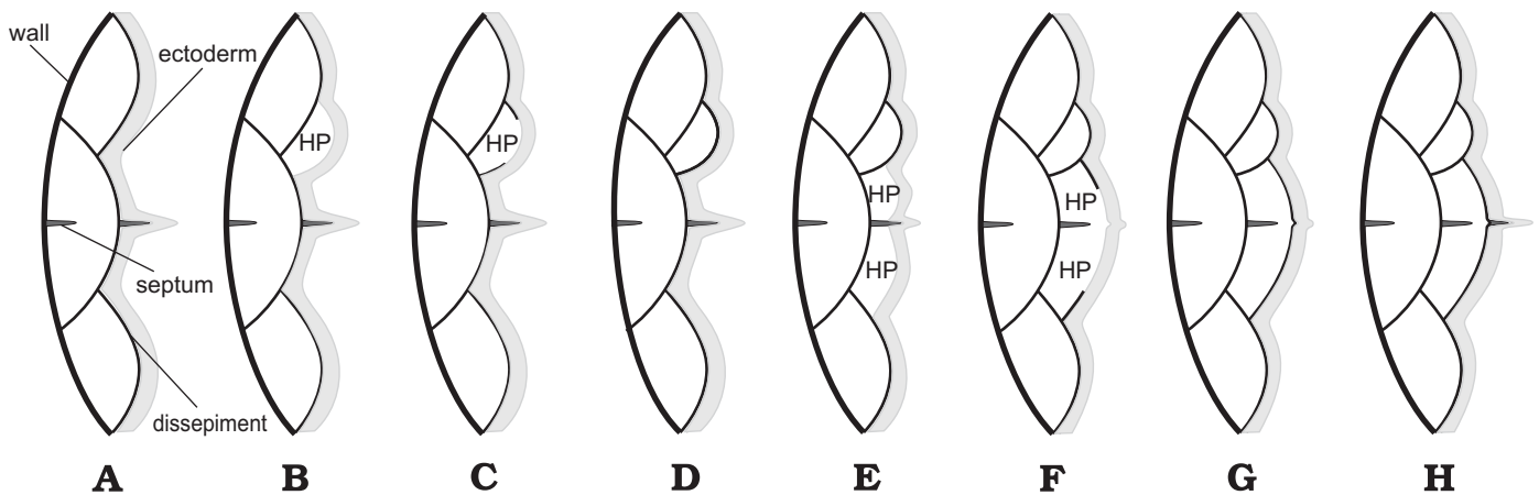
Fig. 6. Schematic drawing showing successive stages of formation of lonsdaleoid dissepiments. A–D. Smaller dissepiment created between septal pockets. E–H. Larger dissepiment created in place with septal pocket, disrupting septal growth. Note hydrostatic pressure (HP) between basal ectoderm and skeletal structures is here responsible for the pushing up the ectoderm and shaping the dissepiment. Morphological nomenclature refers to all figures (A–H).
