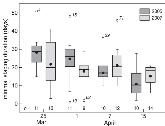
Figure 5. Minimal staging duration (the time interval between tagging and the last recording) of adult male Ruffs radio-tagged in 2005 and 2007. Sample sizes are indicated below box plots. Boxes represent the 95% CI intervals, horizontal lines represent the median, bars represent the range, solid dots are mean values and open dots are outliers.
