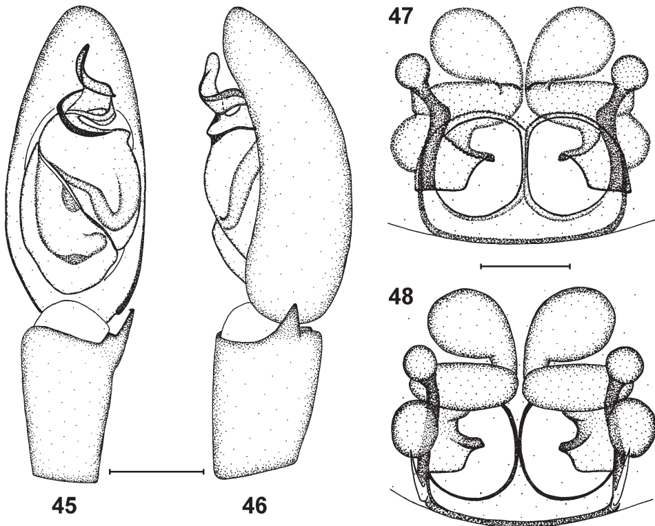
Figs 45–48. Fuchiba venter sp. n.: (45, 46) male palp, ventral and retrolateral views; (47, 48) female epigyne, ventral and dorsal views. Scale bars = 0.1 mm.
