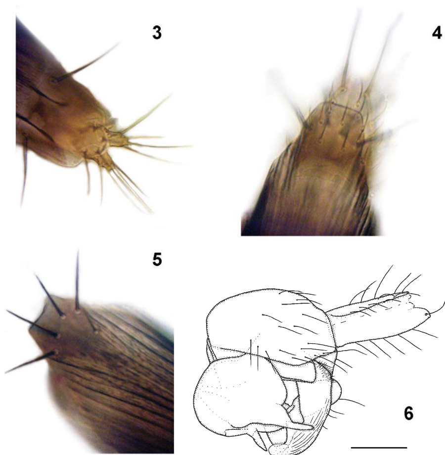
Figs 3–6. Megaselia cakpoe sp. n., ♀ (3–5) and ♂ (6): (3) epiproct and cerci, (4, 5) lobe at rear of sternum 8 in two different specimens, (6) left face of hypopygium. Scale bar = 0.1 mm.
