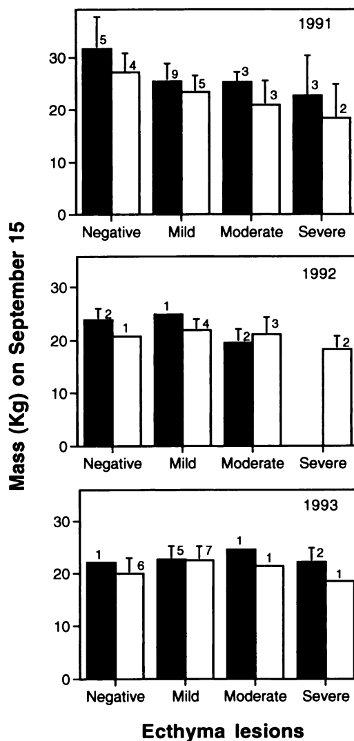
FIGURE 1. Body mass (mean + SD) adjusted to September 15 for bighorn sheep lambs at Ram Mountain, Alberta, Canada, 1991 to 1993, as a function of severity of contagious ecthyma lesions. Numbers above histograms are sample size. Black bars are for male lambs, open bars are for female lambs.
