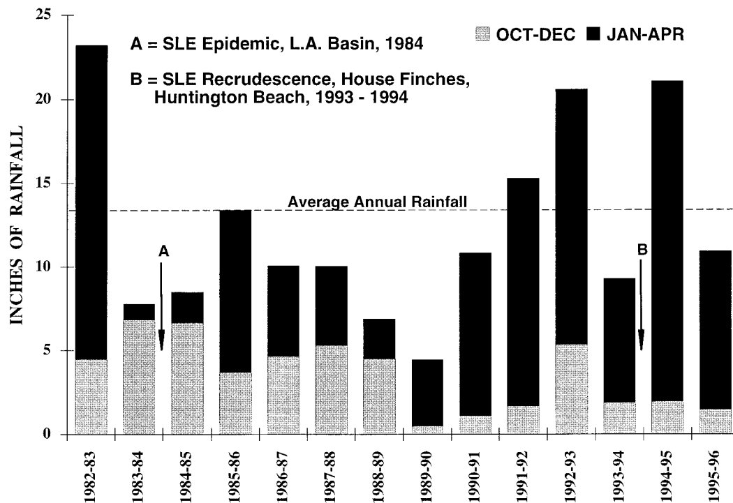
FIGURE 9. Average seasonal rainfall in Orange County, 1982-96; NOAA records.
