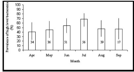
FIGURE 6. Monthly prevalence of a high level of bacteremia in Bartonella -positive Richardson's ground squirrels for all years combined. Error bars represent 95% confidence intervals. Sample size is shown inside column.
