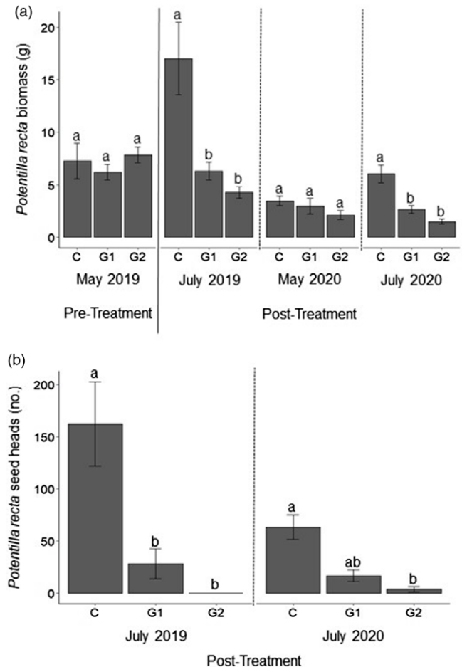
Figure 1. Potentilla recta aboveground biomass (A) pre- and posttreatment and number of seed heads (B) posttreatment at Wycliffe separated by month/year and treatment (C, control; G1, grazing once; G2, grazing twice). Bars represent mean with SE. Aboveground biomass and seed heads were influenced by a significant treatment by month/year interaction ( P < 0.05 ; ANOVA on linear mixed models). Comparisons between treatments within a given month/year are shown with different letters indicating significant differences.
