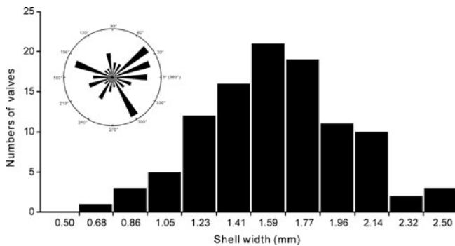
Figure 16. Size frequency distribution and rose diagram of Linnarssonina sapushanensis from the lower Cambrian Shipai Formation at Xiachazhuang section, Three Gorges area, South China.
