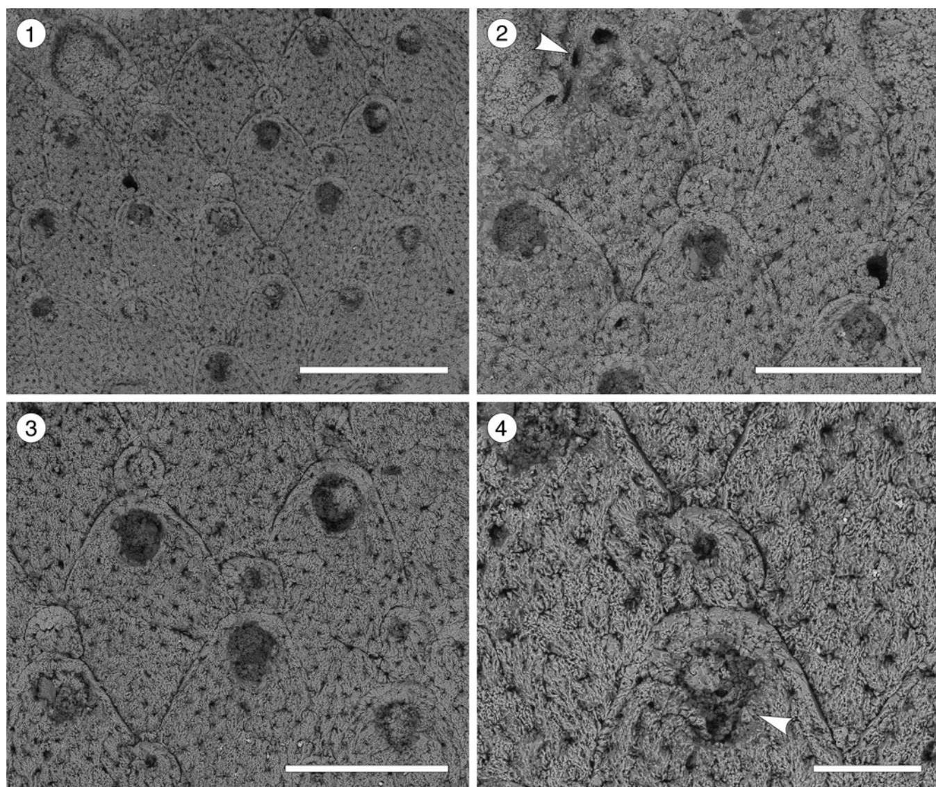
Figure 3. Trypostega sp. indet. (MUN-STRI-47675) from the Siamaná Formation, Arroyo Uitpa. (1) General view of the zooids; (2) detail of the basal pore-chambers (arrowed); (3) detail of the zooids and zooeciules; (4) detail of the orifice, sinus, and likely condyles (arrowed). Scale bars are (1) 0.5 mm; (2, 3) 0.3 mm; (4) 0.1 mm.
