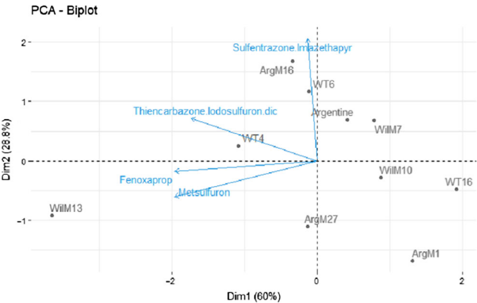
Figure 2. Principal component analysis (PCA) of metsulfuron, fenoxaprop, sulfentrazone + imazethapyr, and thien carbazon + iodosulfuron + dicamba, performed to identify genotype clustering using the singular-value decomposition method. Two-dimensional plot (Dim1 vs. Dim2). The response variable used in the PCA was % plant growth 30 d after treatment (means averaged across 1× and 2× rates). Genotypes are shown as loadings and represented with dots. Herbicides are shown as vectors and represented with blue arrows.
