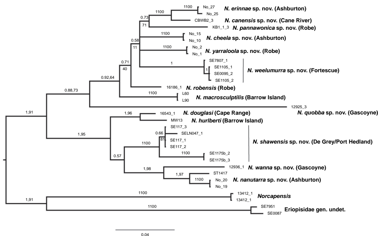
Fig. 2. Maximum Likelihood (ML) phylogeny of Nedsia species based on COI +28S combined analysis. Numbers on branches represent posterior probabilities from Bayesian Inference (left hand side) and ML bootstrap values as a percentage (right hand side).
