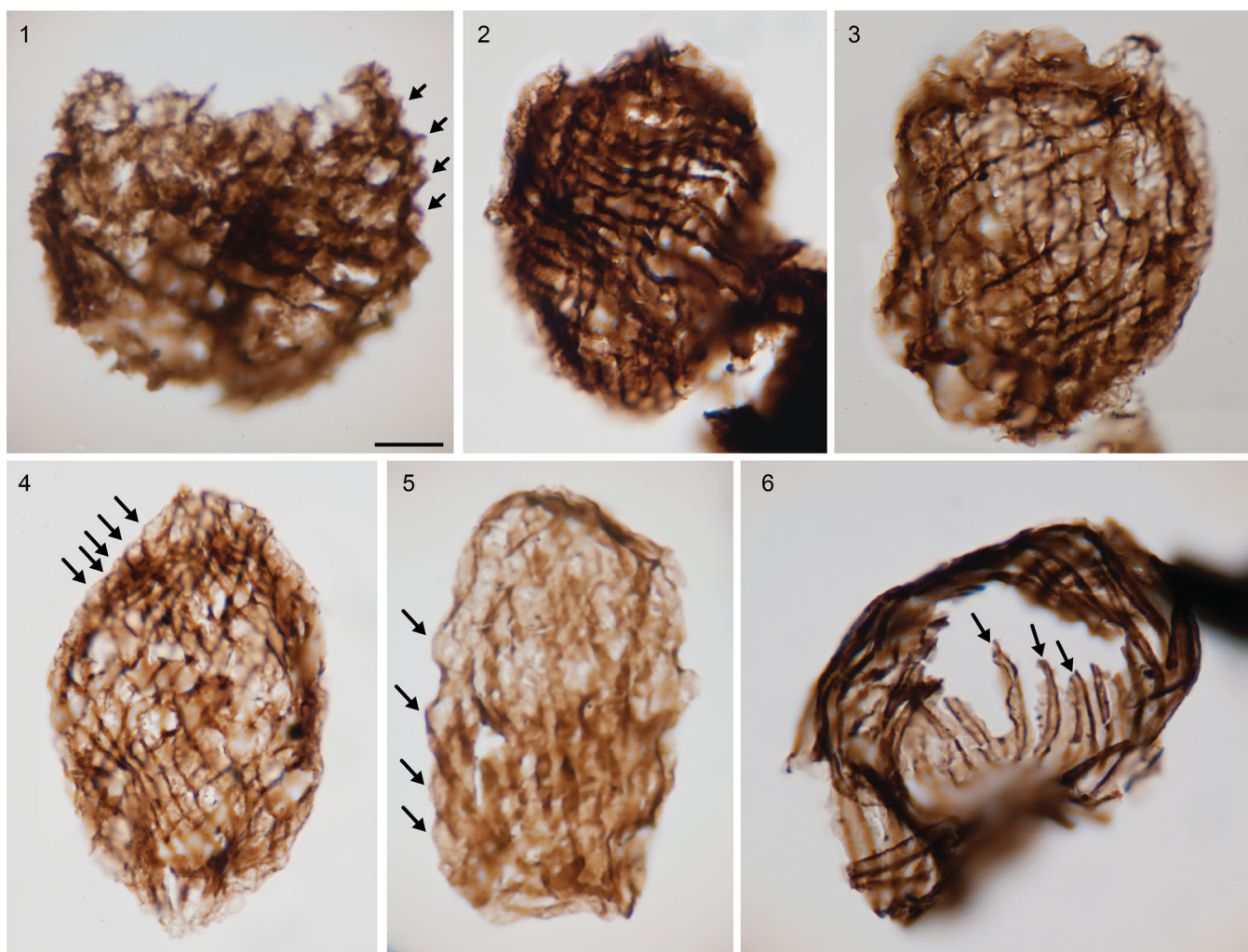
Plate 1. Transmitted white light micrographs of Moyeria sp. and M. cabottii from the Upper Silurian of the Hagshaw Hills inlier. All specimens are from sample CH1 collected from the Glenbuck Loch locality, sample 12CW156, slide BH4/1. Scale bar in 1 = 10 \mu m in all images. Slide loc. refers to England Finder coordinates. Figure 1. A nearly spherical specimen showing distinctly serrated/crenulate margin where strips wrap around the cell (arrows), loc. ca. H20. Figure 2. A typical prolate specimen, loc. L51. Figure 3. This squarish specimen clearly shows the cross-hatched nature of the compressed top and bottom walls, loc. L61. Figure 4. A sub-fusiform specimen with crenulated margin where pellicle strips wrap around the cell (arrows), loc. Q43. Figure 5. A subrectangular form with somewhat wider pellicle strips and distinctly crenulated margin (arrows), loc. D21. Figure 6. A damaged specimen with distinctive, wider pellicle strips. Individual strips are discernible in the centre of the specimen (arrows) where it is broken and only a single layer of the pellicle is present and unobscured by the opposing layer, loc. T59.
