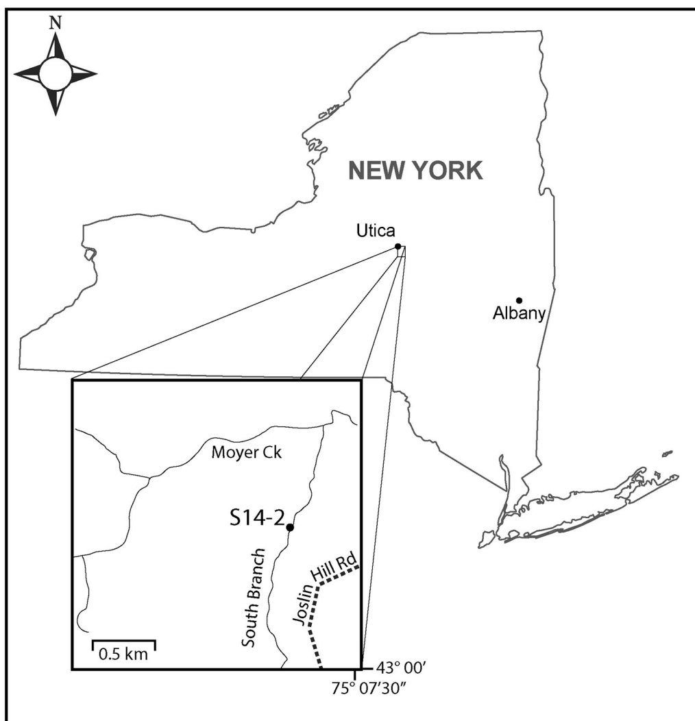
Figure 2. Location map for the section along the south branch of Moyer Creek, New York State, located in the SE quadrant of the Utica East USGS Quadrangle. Sample S14-2 is located at 43°0.5835'N 75°7.8618'W. Source: Authors.
