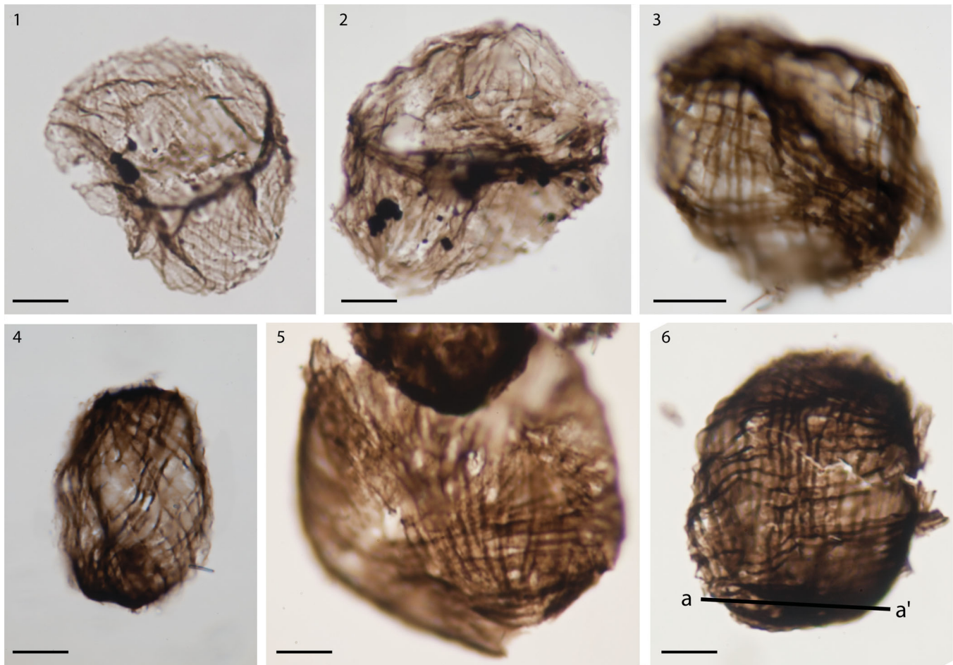
Plate 3. Transmitted white light micrographs of Moyeria from the type section along the south branch of Moyer Creek, New York State, USA. Scale bar = 10 µm in all images. Slide loc. refers to England Finder coordinates. Figure 1. A globular specimen of Moyeria uticana Thusu that clearly shows the diamond-shaped cross-hatching that characterises this taxon. It also shows the rucked-up, thickened bands that form during compression and traverse the entire specimen. This specimen is quite similar in all aspects to the holotype (Thusu 1973, plate 2, figure 19). Sample S14-2/10, loc. M33. Figure 2. This additional example of a globular M. uticana is similar in appearance to the holotype. This photograph is a montage of different focal planes. Sample S14-2/7, loc. D34. Figure 3. Another roughly spherical to globular specimen of M. uticana . Sample S14-2/11. Figure 4. A prolate form of Moyeria sp., which is smaller than the more globular forms that are closer in form to the holotype of M. uticana . This photograph is a montage of different focal planes. Sample S14-2A/2, loc. U29. Figure 5. This nearly spherical form, which is nearly 60 µm in diameter, is slightly larger than the typical M. uticana specimens illustrated in Thusu (1973). Sample S14-2/6, loc. E36. Figure 6. A somewhat ellipsoidal specimen of Moyeria uticana . Line a–a' shows the approximate line of section for the transmission electron microscopy image in Plate 4, figure 1. Sample S14-2/1, loc. P30.
