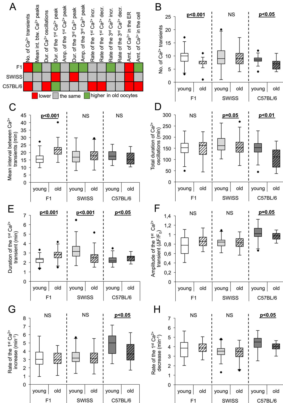
Figure 1. Effect of maternal aging on the pattern of fertilization-induced \text{Ca}^{2+} oscillations in oocytes from F1, SWISS, and C57BL/6 mice. (A) Summary of the alterations induced by maternal aging in \text{Ca}^{2+} oscillations in fertilized oocytes. Red marks values lower, gray—the same, and green—higher in old oocytes than in their young counterparts. The amounts of \text{Ca}^{2+} in the ER and the whole cell correspond to the AUCs for the TG- and A23187-induced \text{Ca}^{2+} increases, respectively. (B) The number of \text{Ca}^{2+} transients in young ( n = 57 F1, 93 SWISS, 36 C57BL/6) and old ( n = 30 F1, 74 SWISS, 17 C57BL/6) oocytes. (C) Mean interval between two consecutive \text{Ca}^{2+} transients calculated for the first 2 h of \text{Ca}^{2+} oscillations in young ( n = 57 F1, 92 SWISS, 36 C57BL/6) and old ( n = 29 F1, 74 SWISS, 17 C57BL/6) oocytes. (D) The total duration of \text{Ca}^{2+} oscillations in young ( n = 57 F1, 92 SWISS, 36 C57BL/6) and old ( n = 29 F1, 74 SWISS, 17 C57BL/6) oocytes. (E) Duration and (F) amplitude of the 1st \text{Ca}^{2+} transient in young ( n = 55 F1, 92 SWISS, 36 C57BL/6) and old ( n = 27 F1, 73 SWISS, 18 C57BL/6) oocytes. (G) Rate of \text{Ca}^{2+} increase during the 1st \text{Ca}^{2+} transient in young ( n = 54 F1, 92 SWISS, 36 C57BL/6) and old ( n = 27 F1, 74 SWISS, 18 C57BL/6) oocytes. (H) Rate
