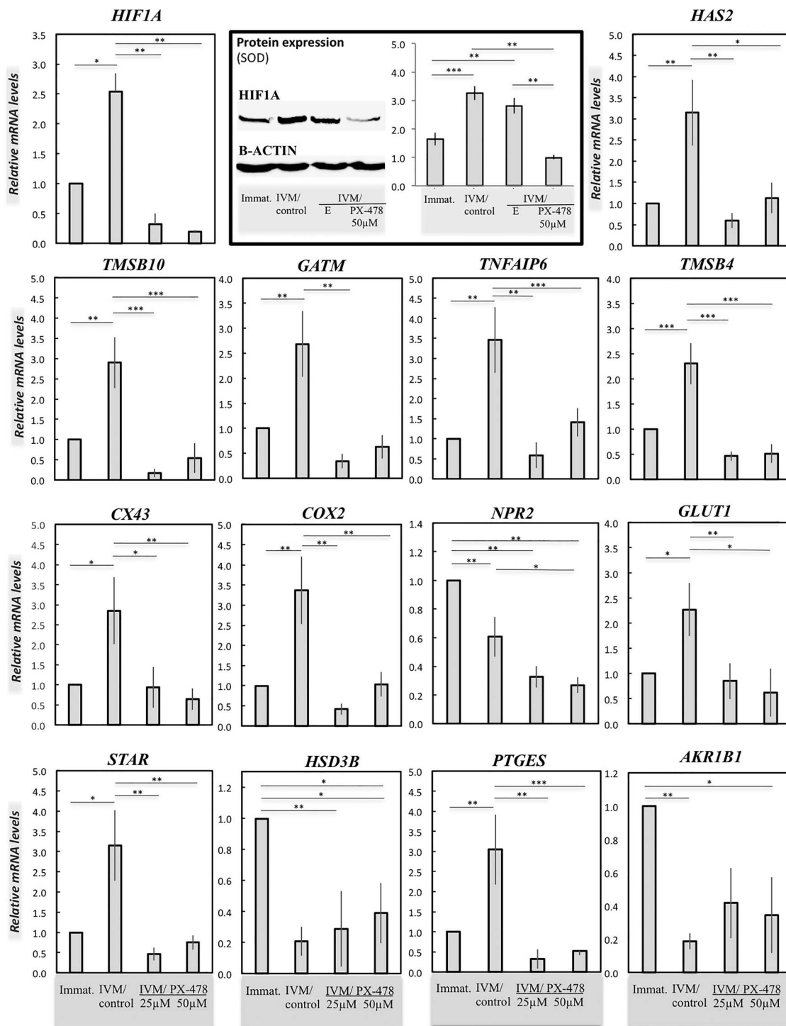
Figure 4. Effects of the suppression of HIF1 \alpha expression by PX-478 on target gene expression in cumulus cells derived from COCs as evaluated by semi-quantitative (TaqMan) real time PCR. The following experimental groups were involved: immature COCs (Immat.), control in vitro matured COCs (IVM/control), and COCs treated with two dosages of PX-478 (25 and 50 \mu M) during IVM (IVM/25 \mu M PX-478 and IVM/50 \mu M PX-478). The one-way ANOVA was applied to test the effect of HIF1 \alpha suppression on gene expression in treated cells, revealing: HIF1A ( P = 0.0016 ), HAS2 ( P = 0.018 ), TNFAIP6 ( P = 0.0006 ), TMSB4 ( P < 0.0001 ), TMSB10 ( P = 0.0002 ), GATM ( P = 0.002 ), NPR2 ( P < 0.0001 ), GLUT1 ( P = 0.004 ), CX43 ( P = 0.06 ), COX2 ( P = 0.001 ), PTGES ( P = 0.005 ), AKR1B1 ( P = 0.004 ), STAR ( P = 0.002 ), and HSD3B ( P = 0.002 ). Additionally, the HIF1 \alpha protein levels were determined by Western blot analysis in all experimental groups, i.e., immature, as well as in control and PX-478 (50 \mu M) and echinomycin (5 nM) treated IVM groups. The one-way ANOVA was applied revealing P < 0.0001 . Tukey–Kramer multiple comparisons post-test was applied to test the effect of treatment on gene and/or protein expression (solid lines). Bars with asterisks differ at: * P < 0.05 , ** P < 0.01 , *** P < 0.001 , as indicated on the figure. Results are presented as mean \pm SEM.
