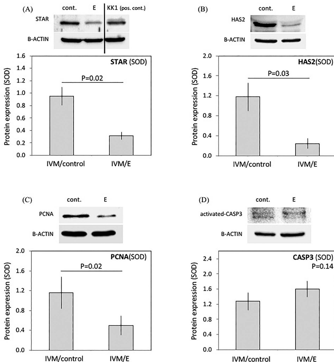
Figure 5. Effects of functional HIF1 \alpha suppression on protein expression of STAR, HAS2, PCNA, and activated-CASP3 in cumulus cells. Cumulus cells were collected from COCs matured in vitro in the absence (IVM/control) or presence of echinomycin (5 nM) (IVM/E). Cells were denuded, collected, and homogenized; 25–30 \mu g of total protein were used for Western blot analysis. Representative Western blots are shown. Student t -test, unpaired, two-tailed, was applied; the average standardized optical density is shown (mean \pm SEM) for: (A) STAR 30 kDa, (B) HAS2, 64 kDa, (C) PCNA 29 kDa, and (D) activated-CASP3, 17kDa. B-ACTIN was used as loading control (45 kDa). For STAR expression, mouse granulosa KK1 cells were used [42]. Solid lines placed over bars indicate a statistically significant difference between groups.
