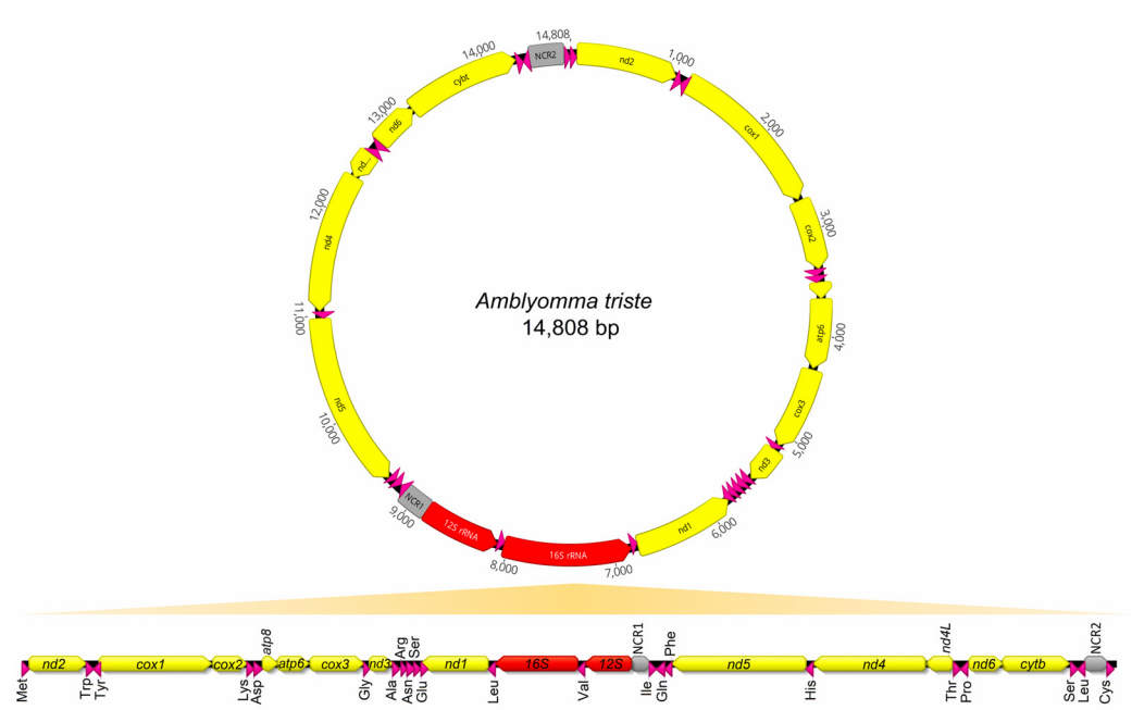
FIGURE 1. Circular and linear representation of the mitochondrial gene order of Amblyomma triste . Gene scaling is approximate, and the end of the arrow indicates the direction of the genes (the genes encoded in the H-strand or “+” and L-strand or “-”). All genes have standard nomenclature including the 22 tRNA genes, which are designated by a three-letter code for the corresponding amino acid. The CDS genes are in yellow, the rRNAs in red, the tRNAs in pinkish-purple color, and the two potential control regions (CR), are non-coding in gray.
