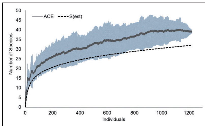
Figure 2. Expected number of species ( S_{est} ; dashed line) and mean ( \pm SD ) abundance coverage-based estimator of species richness (ACE; solid line) for snakes detected during road-kill surveys conducted on both the primary road and secondary roads in the municipalities of Pampa Grande, Mairana, and Samaipata, Florida Province, Santa Cruz Department, Bolivia.
