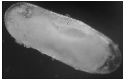
FIGURE 1. Microphotograph of entire egg of Plebeia “nan1,” anterior end upper left.
