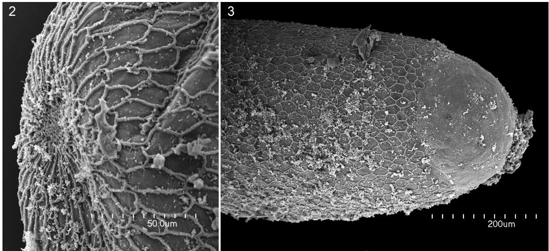
FIGURES 2, 3. SEM micrograph of 2. front and 3. posterior ends of egg of Plebeia "nan1" revealing geometric (mostly hexagonal) chorionic patterning at front and middle of egg and lack of patterning at rear (right).
