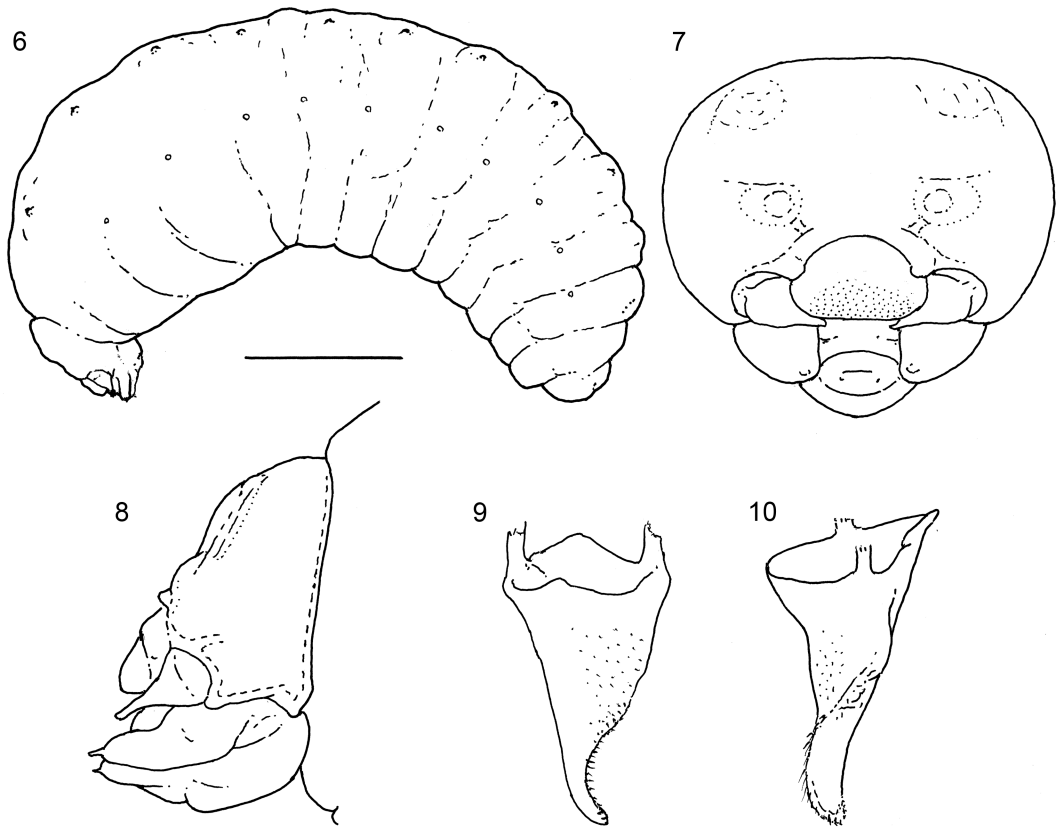
FIGURES 6–10. Diagrams of mature larva of Plebeia “nan1.” 6. Entire larva, with scale bar, lateral view, front end to left. 7, 8. Head, frontal and lateral views. 9, 10. Right mandible, dorsal and inner views.
