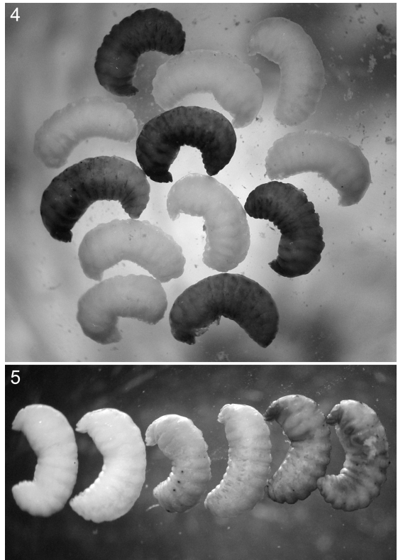
FIGURES 4, 5. Microphotographs of mature postdefecating larvae showing all white, presumable early form, and other various darker forms thought to represent subsequent developmental steps. 4. Mixture of extremes in intensity of darkening. 5. Selection of specimens showing gradations of darkening.
