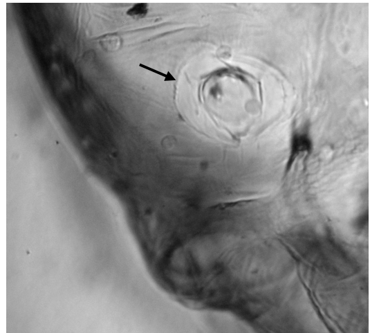
FIGURE 11. Microphotograph of right side of cleared head capsule showing antennal papilla (arrow) surrounded by membranous ring.
