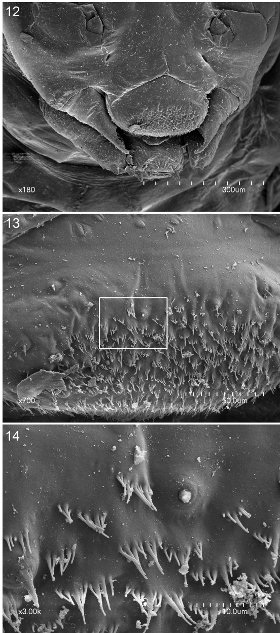
FIGURES 12–14. 12. SEM micrographs of lower part of head, frontal view, showing labrum, with lower, apical part densely spiculate. 13. Close-up of labrum. 14. Close-up of area identified by rectangle in figure 13, showing multipronged spicules.
