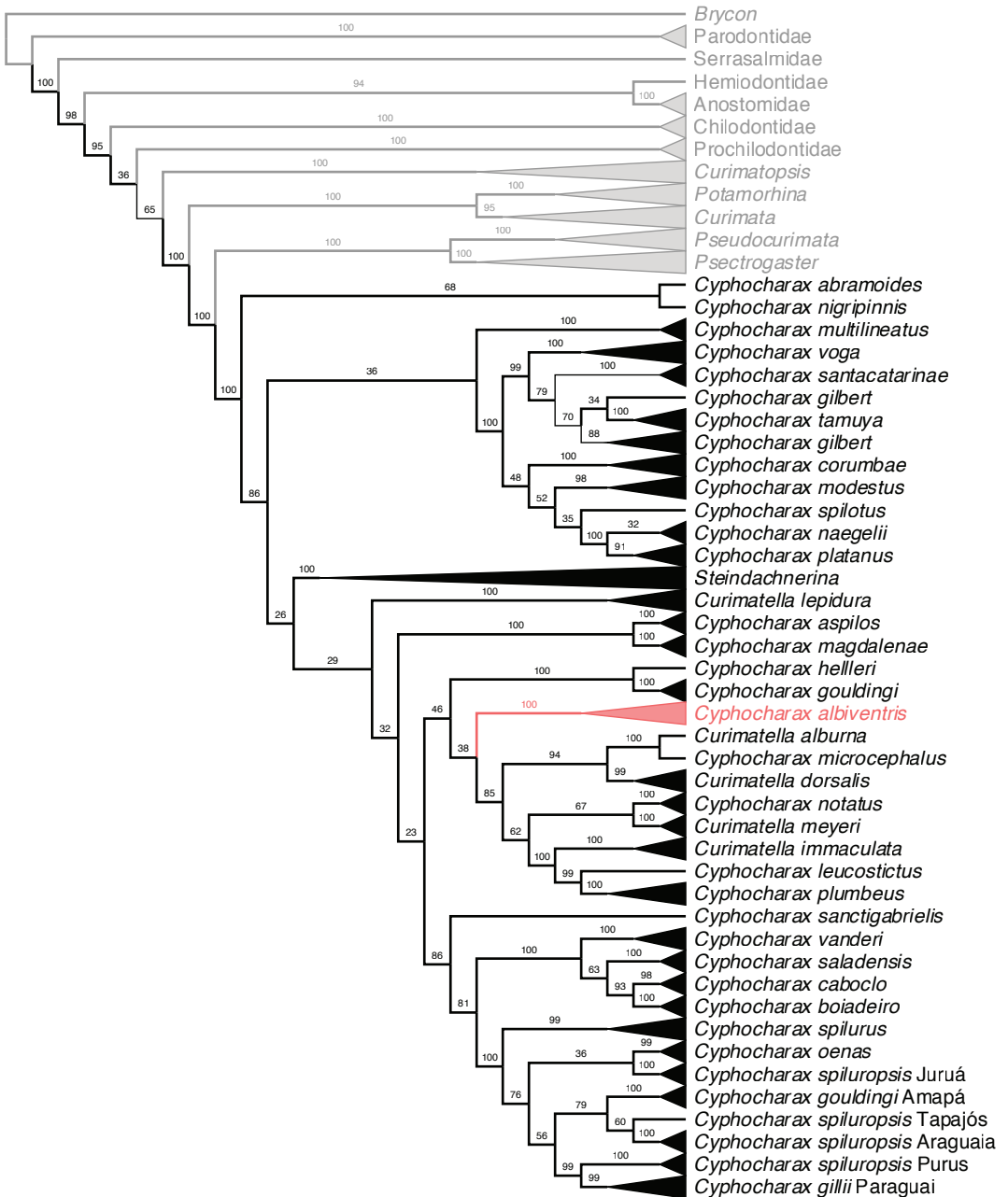
FIG. 3. Maximum-likelihood tree of the multilocus data matrix of Curimatidae highlighting the position of Cyphocharax albiventris within the Curimatella alburna clade. Numbers near nodes represent bootstrap support.
