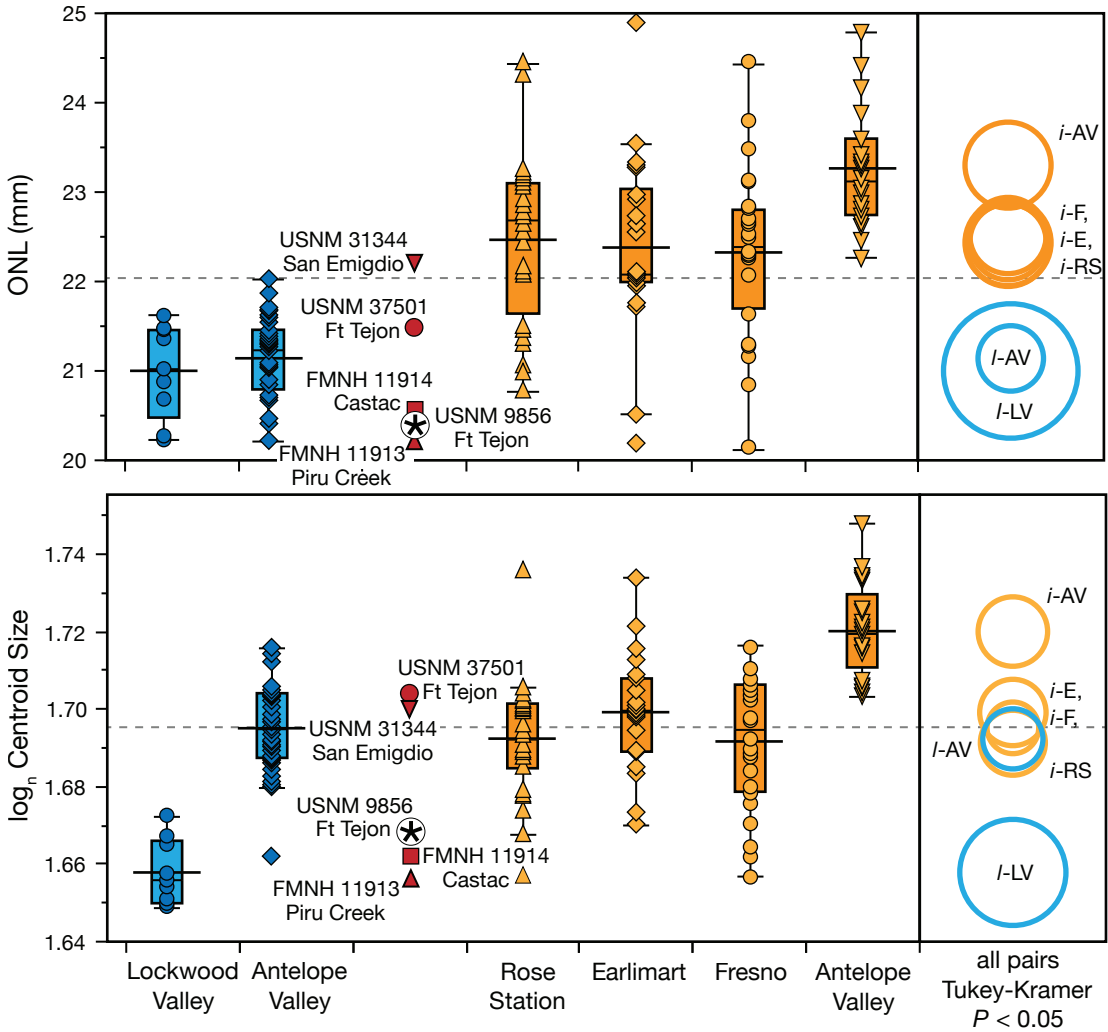
FIG. 4. Box plots of occipito-nasal length (ONL; above) and log n centroid size (logCS; below) for the Osgood Expanded Samples ( longimembris samples in blue; inornatus samples in orange), including sample means and the value placements for each of the five specimens from Fort Tejon and vicinity (white circle with star, USNM 9856/37356, the holotype of longimembris Coues; red circle, topotype USNM 37501; red square, Castac Lake, FMNH 11914; red triangle, Piru Creek, FMNH 11913; and inverted red triangle, San Emigdio, USNM 31344/43209; see maps, fig. 3). The right-hand box contains significant sample subsets (non-overlapping circles) derived from a post-hoc Tukey-Kramer test following the ANOVA comparing all samples (from left to right: i -AV = inornatus Antelope Valley; i -F = Fresno; i -E = Earlimart; i -RS = Rose Station; l -AV = longimembris Antelope Valley; l -LV = Lockwood Valley).
