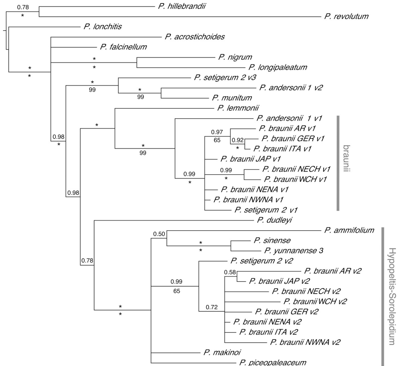
FIG. 5. Phylogram based on combined gapCp and pgcC data. Variants are distinguished with v# suffixes to the accession names. Bayesian posterior probabilities (above branches) and maximum parsimony bootstrap percentages (below branches) given where support values exceed 0.5 or 50% respectively. Asterisk indicates 1.0 PP or 100% BS. AR = Altai, Russia. GER = Germany. ITA = Italy. JAP = Japan. NECH = northeastern China. NENA = northeastern North America. NWA = northwestern North America. WCH = western China.
