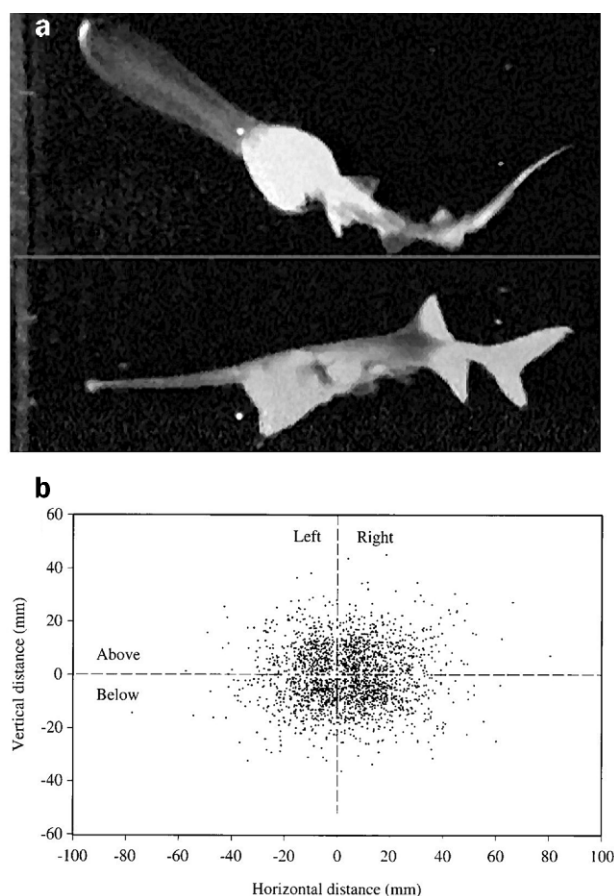
Figure 3. Results from feeding experiments in a flow tank. (a) A video frame with a split image showing lateral (top) and ventral (bottom, via a 45° angled mirror below the chamber) views of the paddlefish. A 90° clockwise roll and yaw response was performed to capture a plankton (view enhanced by a white dot) approaching from above and to the left of the rostrum. The image in the ventral view is reversed by the mirror. (b) For every successful prey capture, the position of the daphnia at the time of first reaction was plotted relative to the midline of the rostrum. Most daphnia were detected at a distance of up to 20 millimeters (mm), but some were as far as 80 mm from the rostrum. Photographs and data: Lon A. Wilkens.
