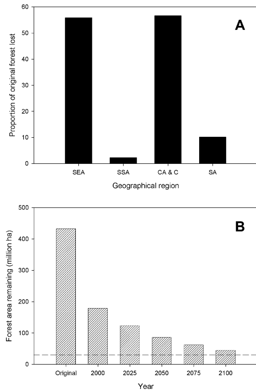
FIG. 2. (A) Comparison of proportion of original forest lost by the year 2000 across tropical regions. Abbreviations: SEA = Southeast Asia, SSA = Sub-Saharan Africa, CA & C = Central America and Caribbean, and SA = South America. (B) Estimated original forest cover, forest cover in 2000, and projected forest cover for Southeast Asia in 2025, 2050, 2075, and 2100 (based on natural forest losses reported by World Resources Institute for 1990–2000). Dashed line represents forest area protected. Data for protected forested areas are from World Resources Institute (see Acknowledgments).
