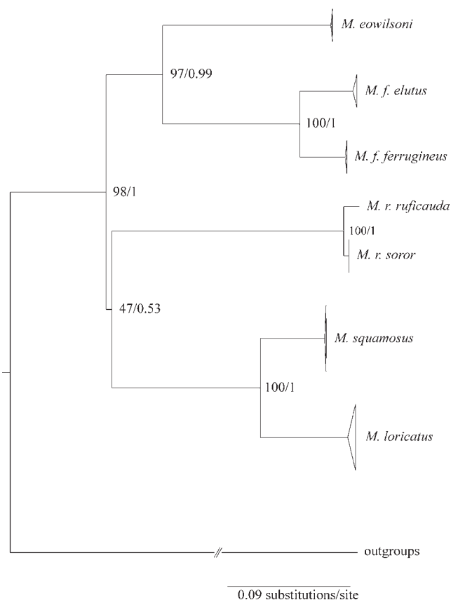
FIGURE 4. Phylogeny of the genus Myrmoderus estimated from a concatenated ND2–ND3 dataset (1,392 bp) using a maximum-likelihood analysis. The Bayesian analysis produced a tree that was topologically identical. Nodal support values are the likelihood bootstrap values and Bayesian posterior probabilities, respectively.
