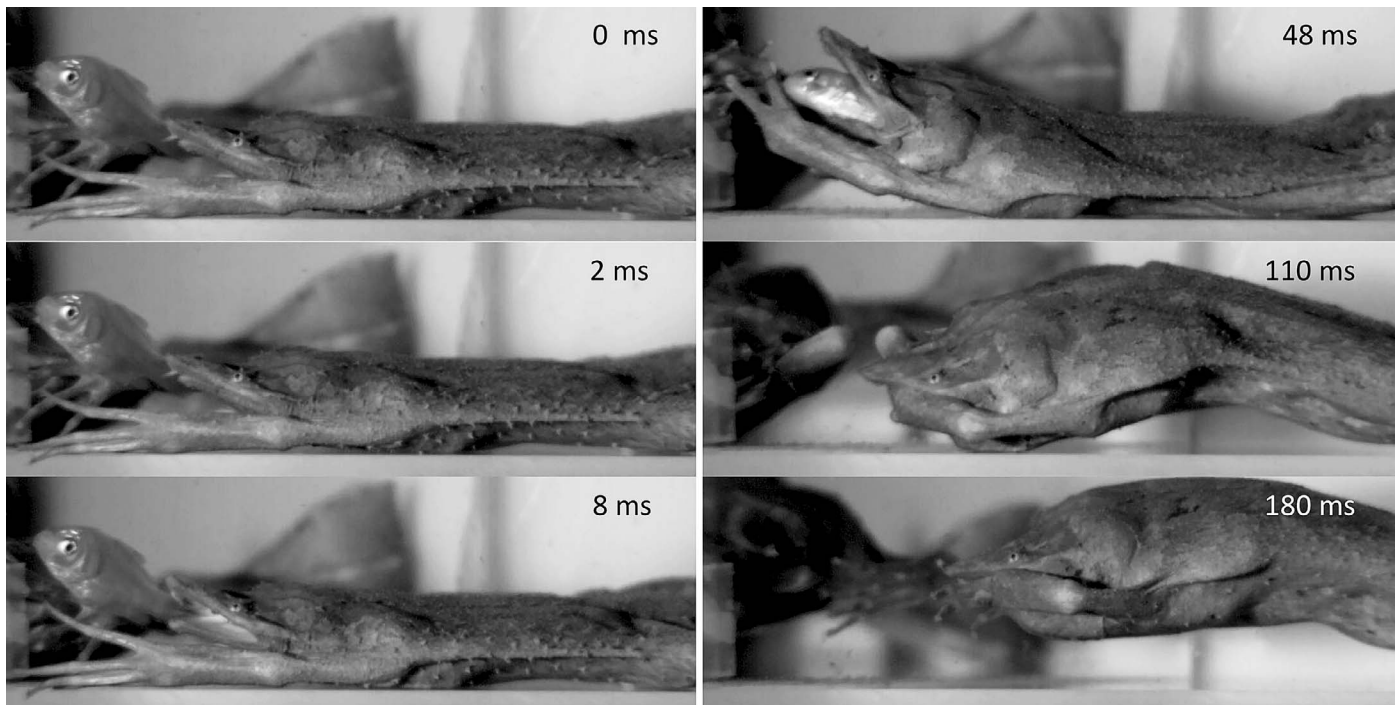
Fig. 2. Six frames from high-speed video of an anterolateral view of a lunging capture of a Carassius auratus by Pipa pipa , showing, at 0 ms, beginning of toe movement; 2 ms, mandible depression; 8 ms, middle of mandible depression, beginning of intraoral suction and forward lunge; 48 ms, beginning of pectoral girdle depression and trunk negative pressure, movement of fish into frog's mouth; 110 ms, dorsal bending of the trunk, continued trunk negative pressure, beginning of reversal of body movement and peak shoulder girdle depression, entry of front feet into mouth, although the fingers did not contact the prey; and 180 ms, inflation of trunk shortly following the end of trunk negative pressure and removal of front feet from mouth.
