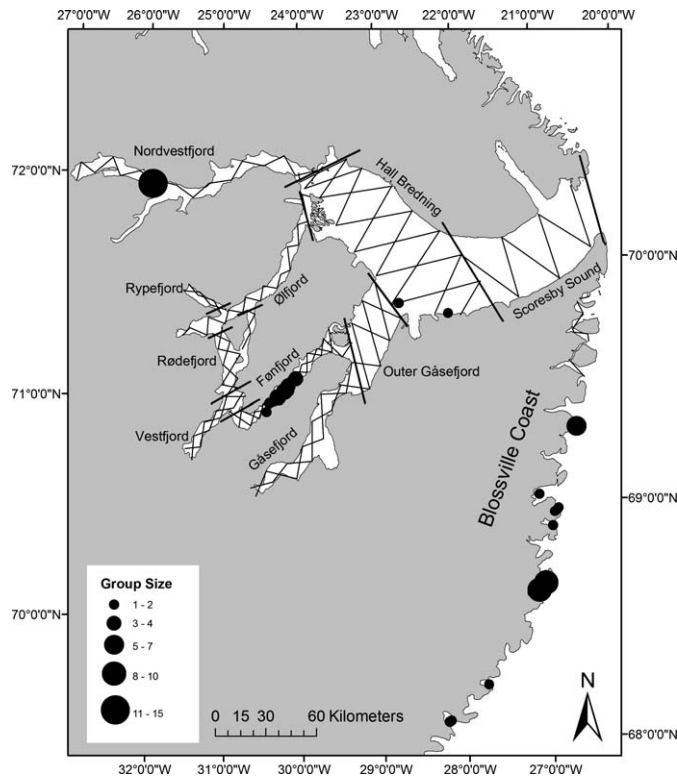
FIG. 4.—Strata with areas, transect lines, and sightings of narwhals in Scoresby Sound and along the northern part of Blosseville Coast during the aerial survey in August 2008.
