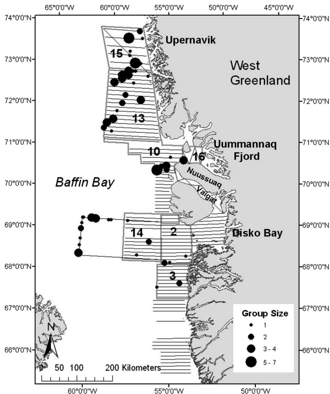
FIG. 2.—Transect lines, strata numbers in bold, and distribution of sightings in the survey of narwhals in West Greenland, March–April 2006.
