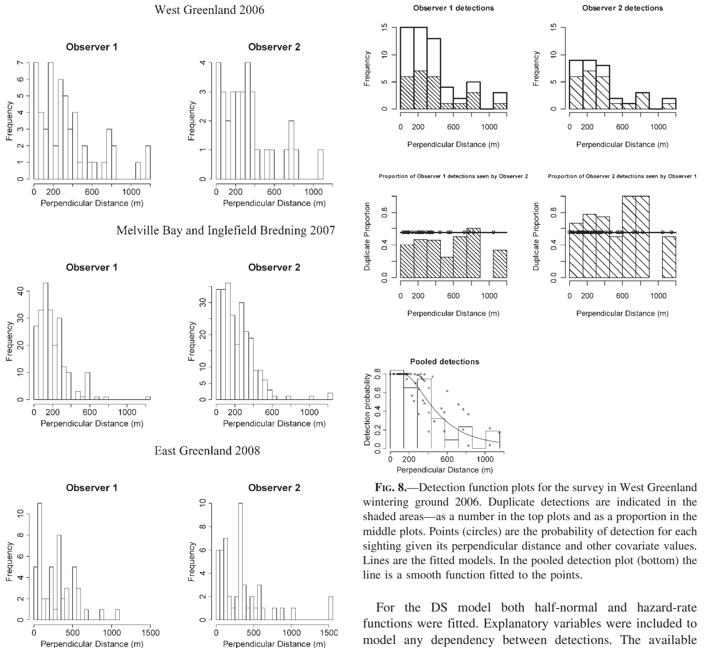
FIG. 7. —Perpendicular distance distributions calculated from the abeam angles recorded by each observer for West Greenland wintering ground (top plots), Melville Bay and Inglefield Bredning (middle), and East Greenland (bottom).
