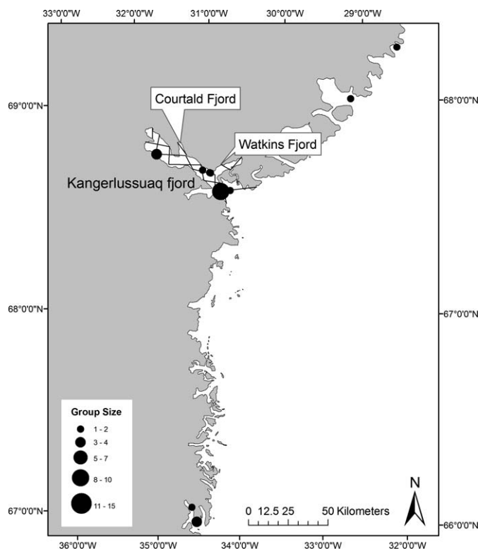
FIG. 5.—Delineation of the strata in Kangerlussuaq and the southern part of the Blosseville Coast, with sightings of narwhals during the survey in August 2008.
