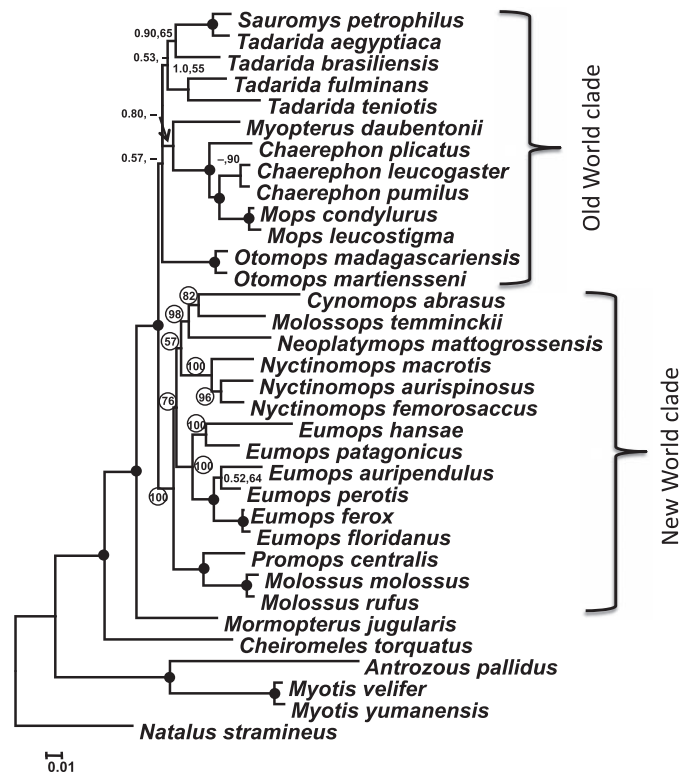
FIG. 7.—Phylogram based on partitioned Bayesian analysis of 4 loci in a combined data set. Support values on branches are Bayesian posterior probabilities (BPPs) followed by bootstrap (BS) values. Solid black dots indicate nodes with BPP \geq 0.95 and BS support \geq 70 . Dashes indicate values less than 50. Circled BPP values are on nodes that were not present in the parsimony tree because of an unresolved position for Nyctinomops aurispinosus , Eumops hansae , and Cynomops abrasus that failed to unite them with other New World taxa.
