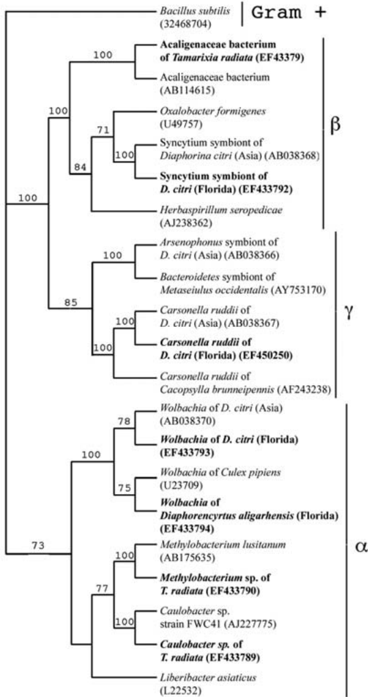
Fig. 1. Phylogenetic tree generated by maximum likelihood analysis based on 16S rRNA sequences from Eubacteria identified from D. citri , T. radiata , and D. aligarhensis compared to related sequences deposited in GenBank. The outgroup taxon is Bacillus subtilis (Gram-positive), and the numbers at branch points of the tree designate bootstrap values. The ingroup taxa are clustered in the \alpha , \beta , and \gamma divisions of the proteobacteria.
