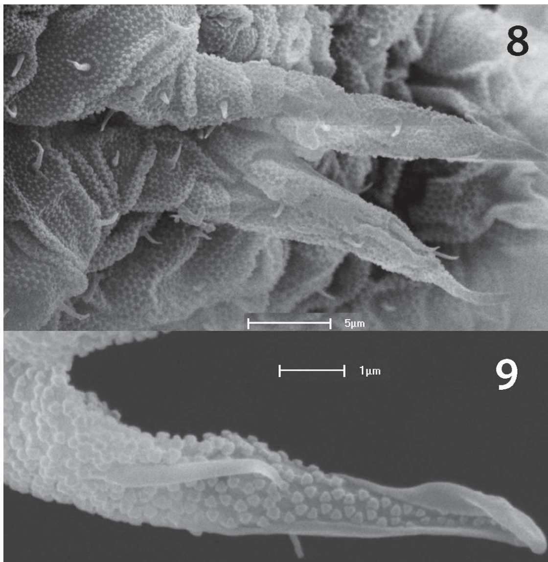
Figs. 8 and 9. Isotogastrura mucrospatulata sp. nov. 8, electro scanning microphotographs of furcula posterior view; and 9, mucro antero-median view.
