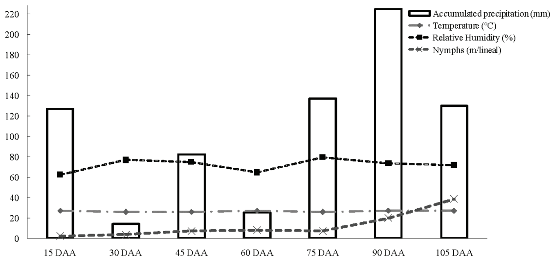
Fig. 1. Cumulative precipitation (mm), average temperature ( ^{\circ}\text{C} ), relative humidity (%) and number of Mah-anarva fimbriolata (Hemiptera: Cercopidae) nymphs in the experimental area at 15 to 105 days after application (DAT) of insect control treatments.
