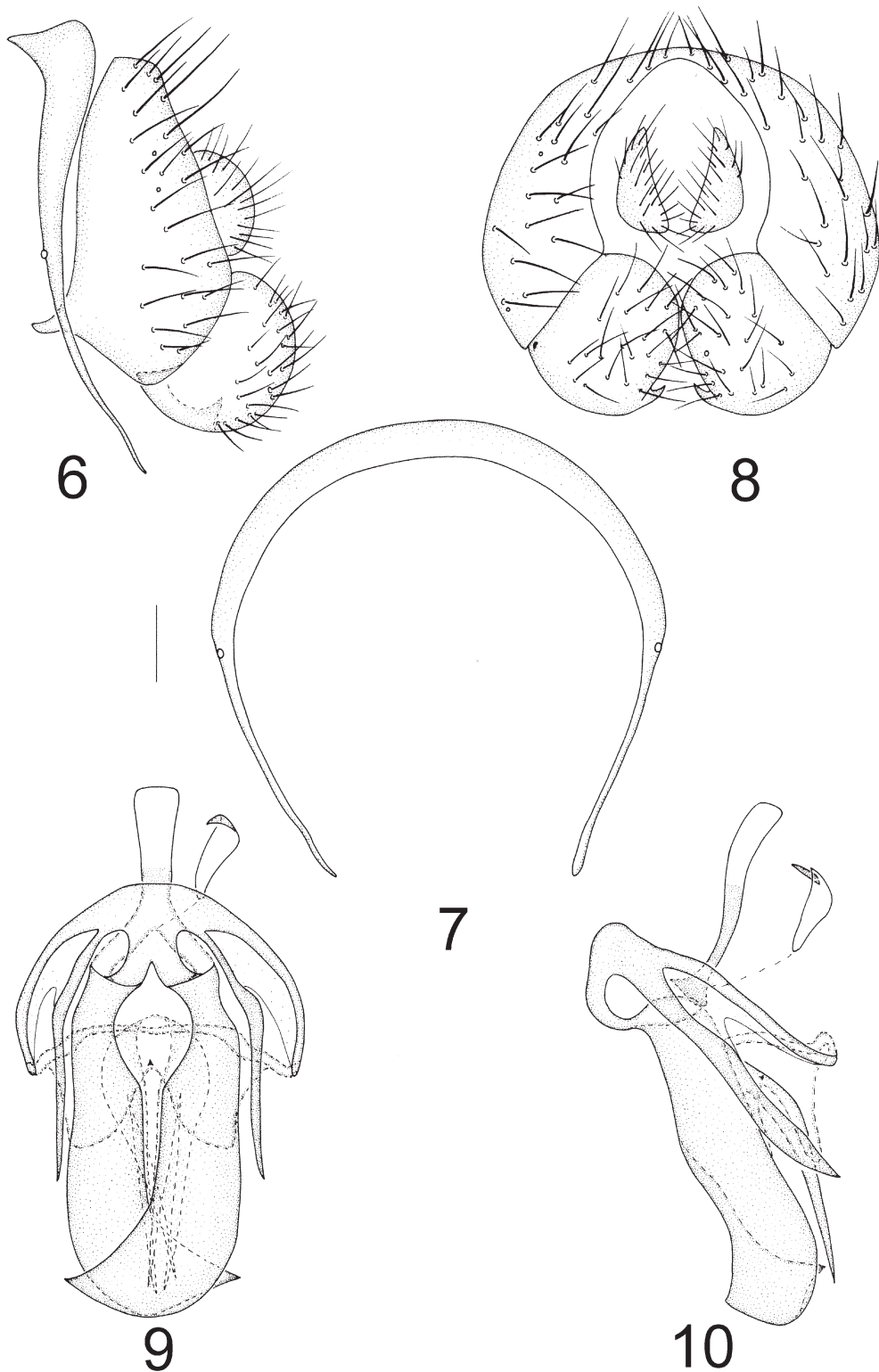
Figs. 6-10. Minettia ( Frendelia ) decussata sp. nov. Male. (6) sytergosternite and epandrium, lateral view; (7) sytergosternite, anterior view; (8) epandrial complex, posterior view; (9) aedeagal complex, ventral view; (10) aedeagal complex, lateral view. Scale bar = 0.1mm.
