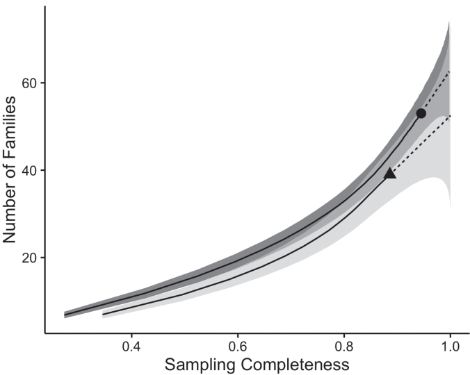
Fig. 1. Sample completeness curve for a vegetable farm (dark shaded area, 38 samples) and blueberry farm (light shaded area, 19 samples) in Suwannee County, Florida. The solid line is the interpolated insect family-level richness and the dashed line is the extrapolated richness. The shaded areas represent 95% confidence intervals. Sampling effort is standardized based on the sample completeness (the proportion of sampled families to predicted families) at each sampling level, with the circle representing final sampling completeness of 38 samples taken at the vegetable farm and the triangle representing final sampling completeness of 19 samples taken at the blueberry farm.
