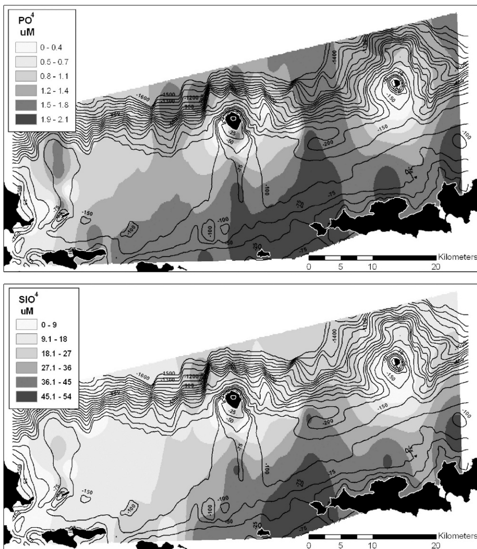
FIGURE 3. Distribution of major nutrients in the Kastochi study area July 2009. Bathymetric contours (m) are displayed for reference. Samples were taken at 10 m depth. See Figure 1 for station locations.
