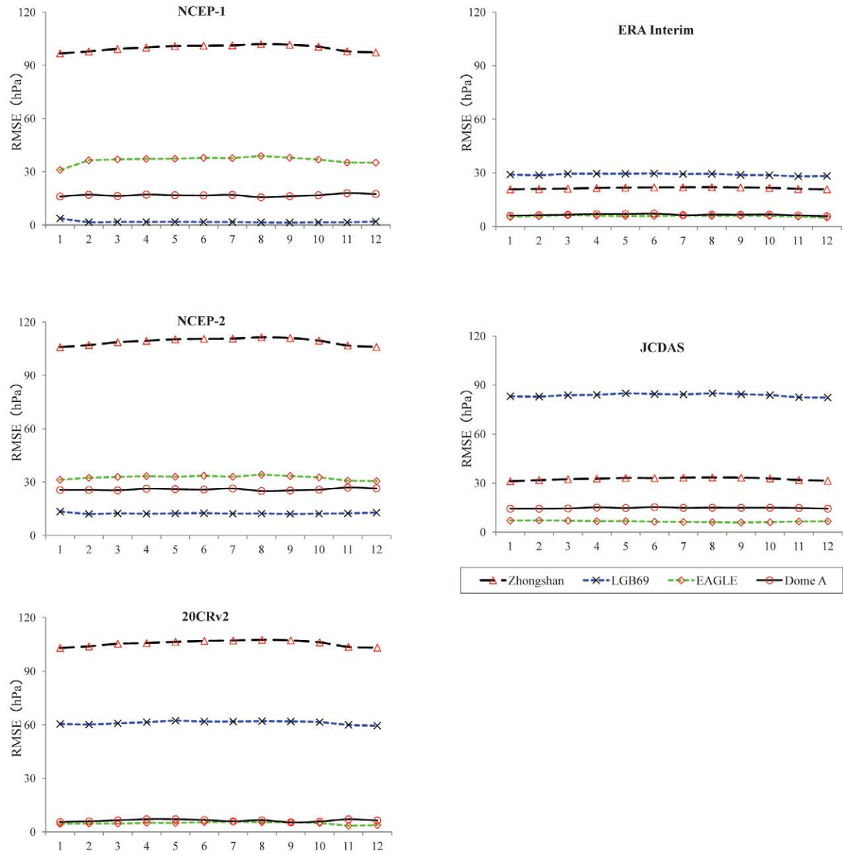
FIGURE 6. Monthly RMSE (hPa) for the reanalyses at the four in situ stations of Zhongshan (black dashed line with red triangle), LGB69 (blue dashed line with cross), EAGLE (green dashed line with red rhombus), and Dome A (black line with red circle).
