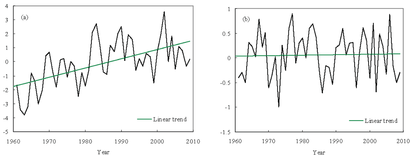
FIGURE 4. The time coefficient of the empirical orthogonal function (EOF) decomposition of the first date of \leq 0 °C temperature: (a) first eigenvector, (b) second eigenvector.
