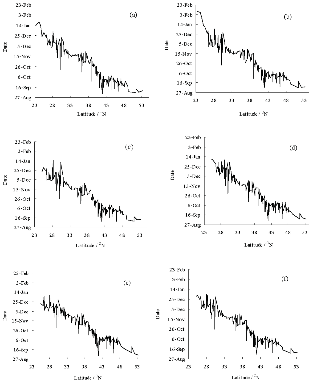
FIGURE 6. The changes in the first date of \leq 0^{\circ}\text{C} temperature within latitude at different time periods: (a) 1960s, (b) 1970s, (c) 1980s, (d) 1990s, (e) 2000s, (f) annual average.
