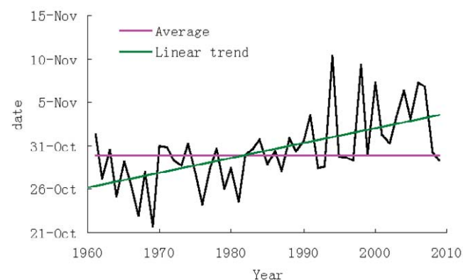
FIGURE 11. The annual average change of the first date of \leq 0^{\circ}\text{C} temperature in East China.
