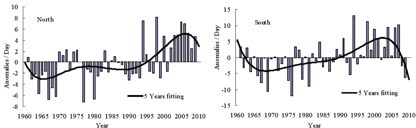
FIGURE 9. Anomalies in the changes of the first date of \leq 0 °C temperature.
