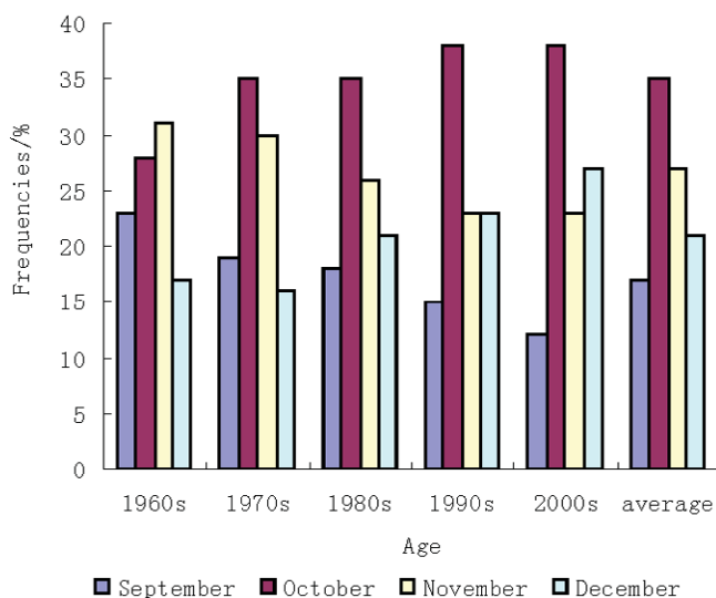
FIGURE 10. The frequencies of the first date of \leq 0^{\circ}\text{C} temperature in different ages.
