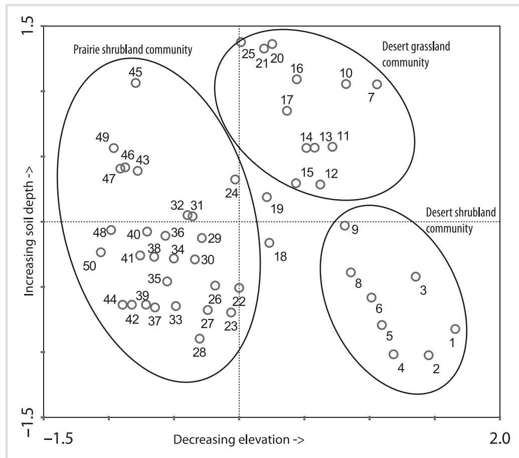
FIGURE 2 Principal component analysis of 50 sample plots on the west slope of the Helan Mountains. The horizontal axis represents a water gradient, with the highest precipitation on the left. The vertical axis represents a soil depth gradient, with higher points on the axis representing an increase in the depth of the soil layer.
