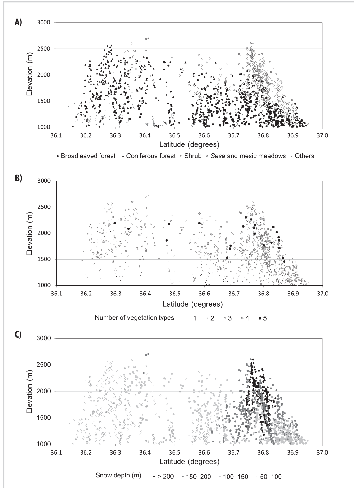
FIGURE 3 (A) Distribution of the most dominant vegetation. (B) Number of vegetation types. (C) Maximum snow depth. The centroids of the polygons are plotted.
