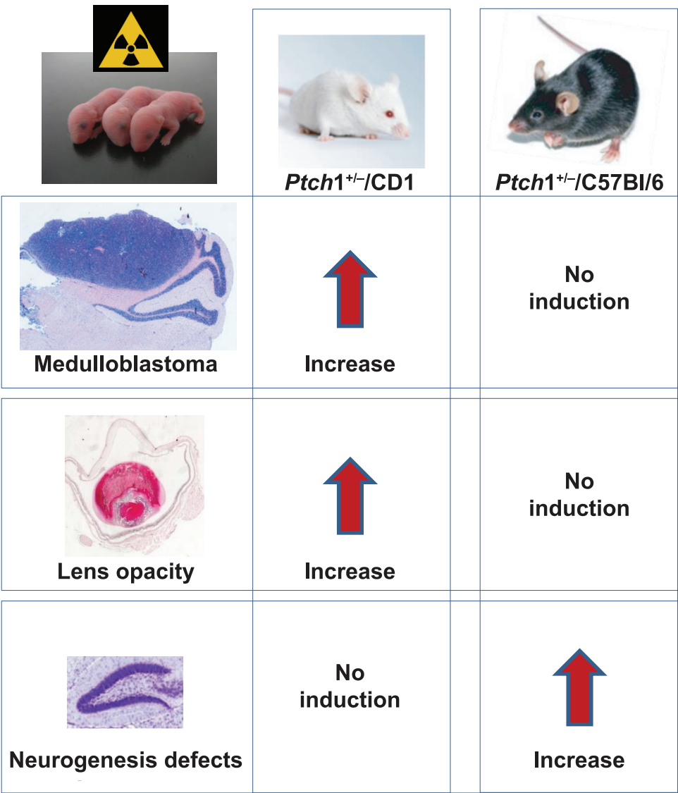
FIG. 7. Schematic representation of the dependence of Ptch1 -associated radiation risk for lens opacity, MB development and neurogenesis defects on mouse genetic background.
