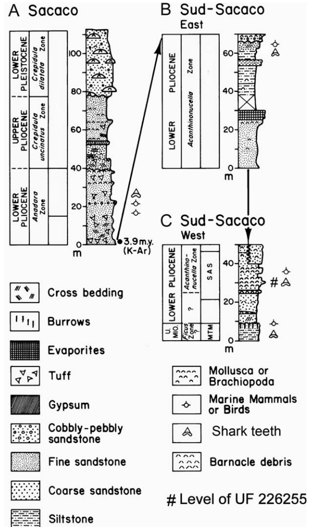
FIGURE 2. Measured sections of Pisco Formation (A–C) in Sacaco basin (from Muizon and DeVries 1985; also see Figure 1) and stratigraphic context (section C) of Carcharodon sp., UF 226255, from early Pliocene Pisco Formation of Peru.
