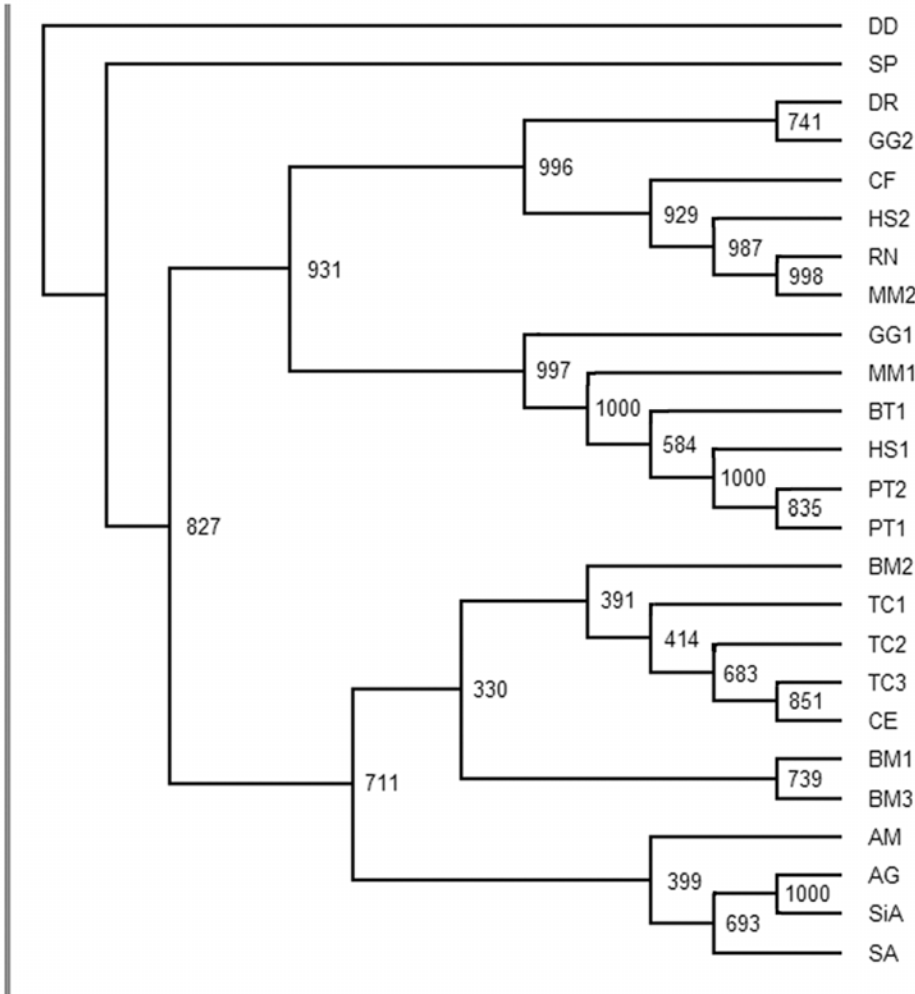
Figure 3. Phylogenetic tree based on amino acid sequences of sid-1-like genes available: DD, Dictyostelium discoideum , GenBank Accession No. XM630477. SP, Strongylocentrotus purpuratus , GenBank Accession No. XP789210. DR, Danio rerio , GenBank Accession No. XM694078. GG2, Gallus gallus , GenBank Accession No. XM001233565. GG1, Gallus gallus , GenBank Accession No. XM416544. CF, Canis familiaris , GenBank Accession No. XM546509. HS1, Homo sapiens , GenBank Accession No. NM017699. HS2, Homo sapiens , GenBank Accession No. NM001040455. RN, Rattus norvegicus , GenBank Accession No. XM001068825. MM1, Mus musculus , GenBank Accession No. NM198034. MM2, Mus musculus , GenBank Accession No. NM172257. BT, Bos taurus , GenBank Accession No. XM585013. PT1, Pan troglodytes , GenBank Accession No. XM001158341. PT2, Pan troglodytes , GenBank Accession No. XM526266. BM1, BM2, BM3, Bombyx mori , cited from George and Gene (2006). TC1, Tribolium castaneum , GenBank Accession No. XM969743. TC2, Tribolium castaneum , cited from George and Gene (2006). TC3, Tribolium castaneum , GenBank Accession No. XM969161. CE, Caenorhabditis elegans , GenBank Accession No. AF478687. AM, Apis mellifera , GenBank Accession No. XM395167. AG, Aphis gossypii , GenBank Accession No. EF533711. SiA, Sitobion avenae , GenBank Accession No. EF533713. SA, Schistocerca americana , GenBank Accession No. AY879097
