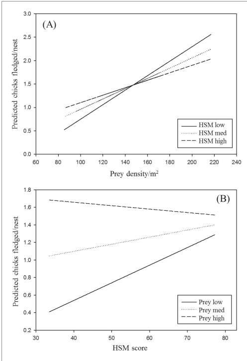
Figure 3. The relationship between predicted wading bird fledging success and (A) prey density at low, medium and high levels of foraging habitat availability (Habitat Suitability Model [HSM]) and (B) foraging habitat availability (HSM Score) at low, medium and high levels of prey density (Prey).
